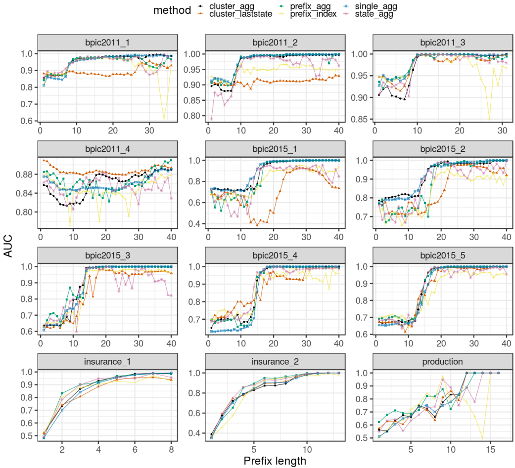
Fig. 7. AUC across different prefix lengths using XGBoost
