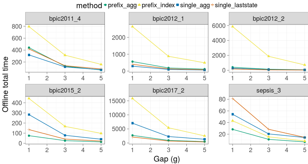
Fig. 9. Offline times across different gaps (XGBoost)
