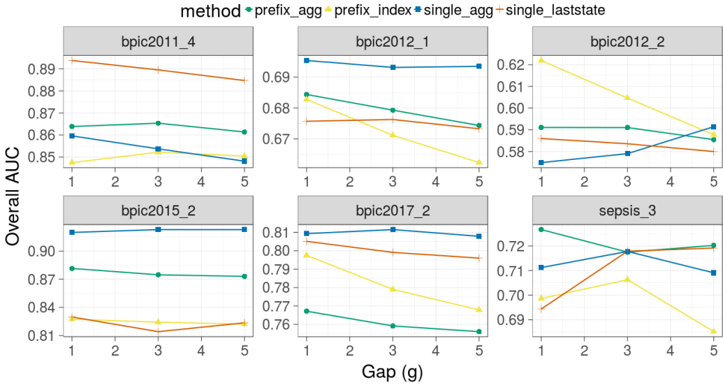
Fig. 10. AUC across different gaps (XGBoost)
