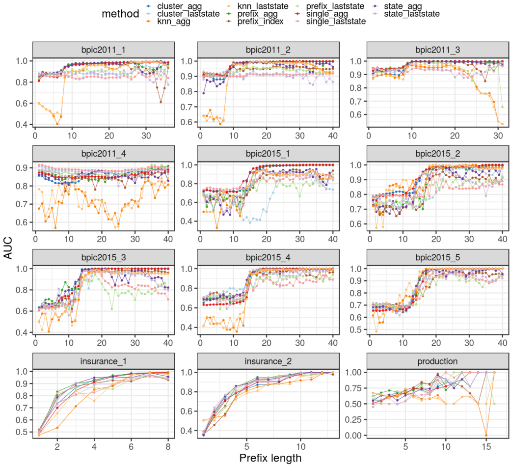
Fig. 19. AUC across prefix lengths using XGBoost, all methods
