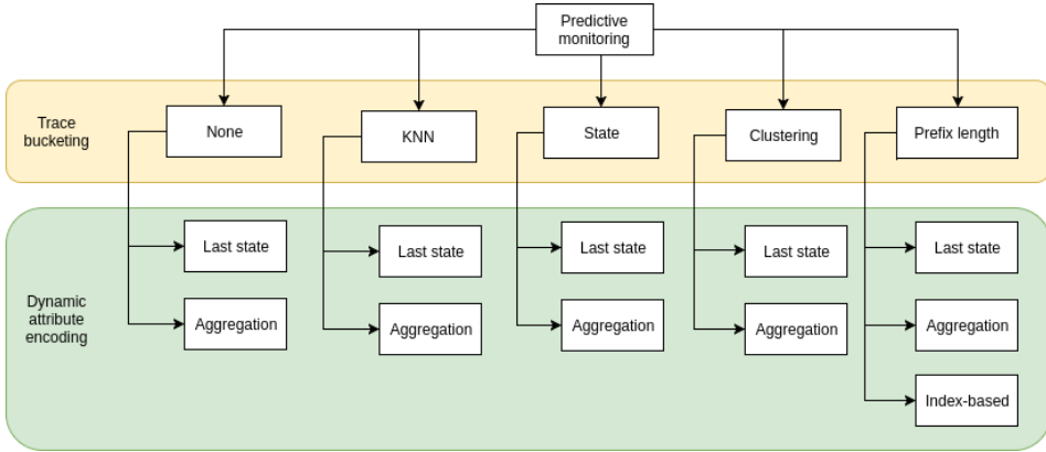
Fig. 4. Taxonomy of methods for predictive monitoring of business process outcome.
