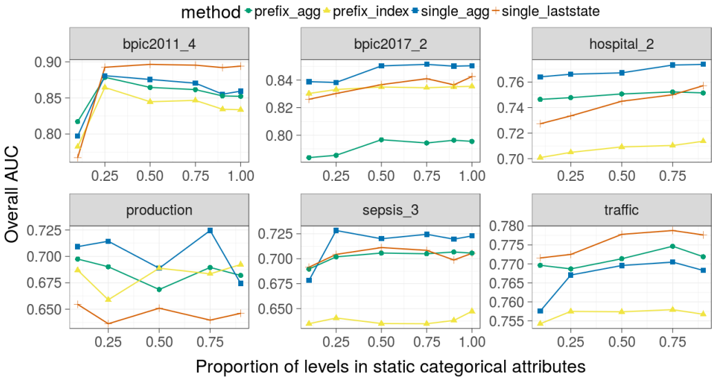
Fig. 26. AUC across different filtering proportions of static categorical attribute levels (XGBoost)
