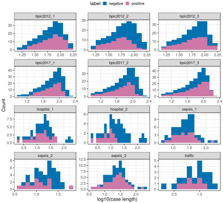
Fig. 16. Case length histograms for positive and negative classes (continued)
