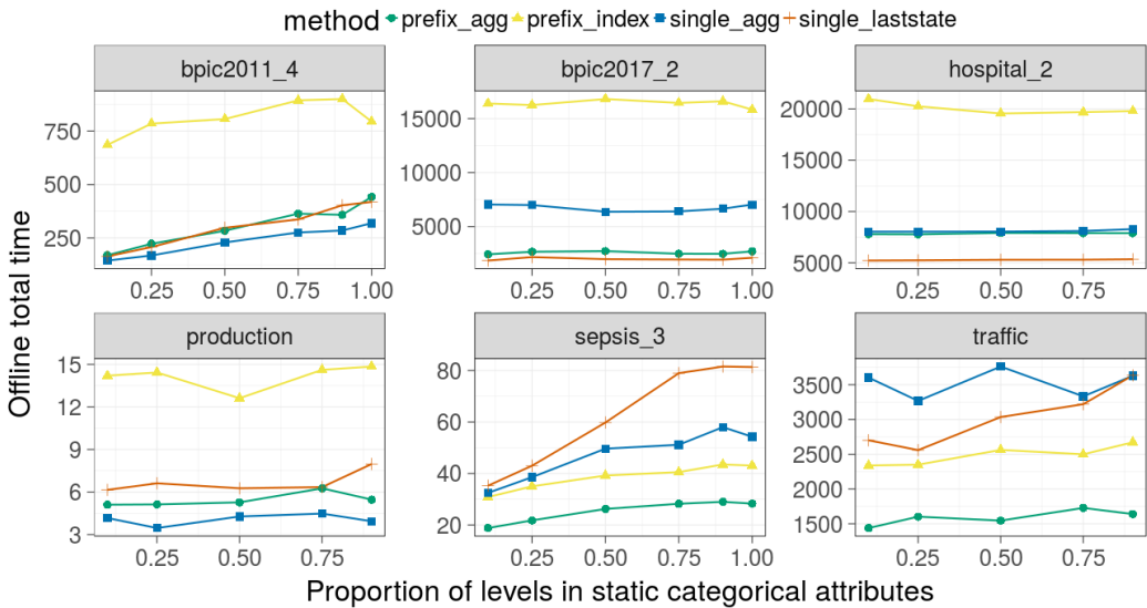
Fig. 24. Offline times across different filtering proportions of static categorical attribute levels (XGBoost)
