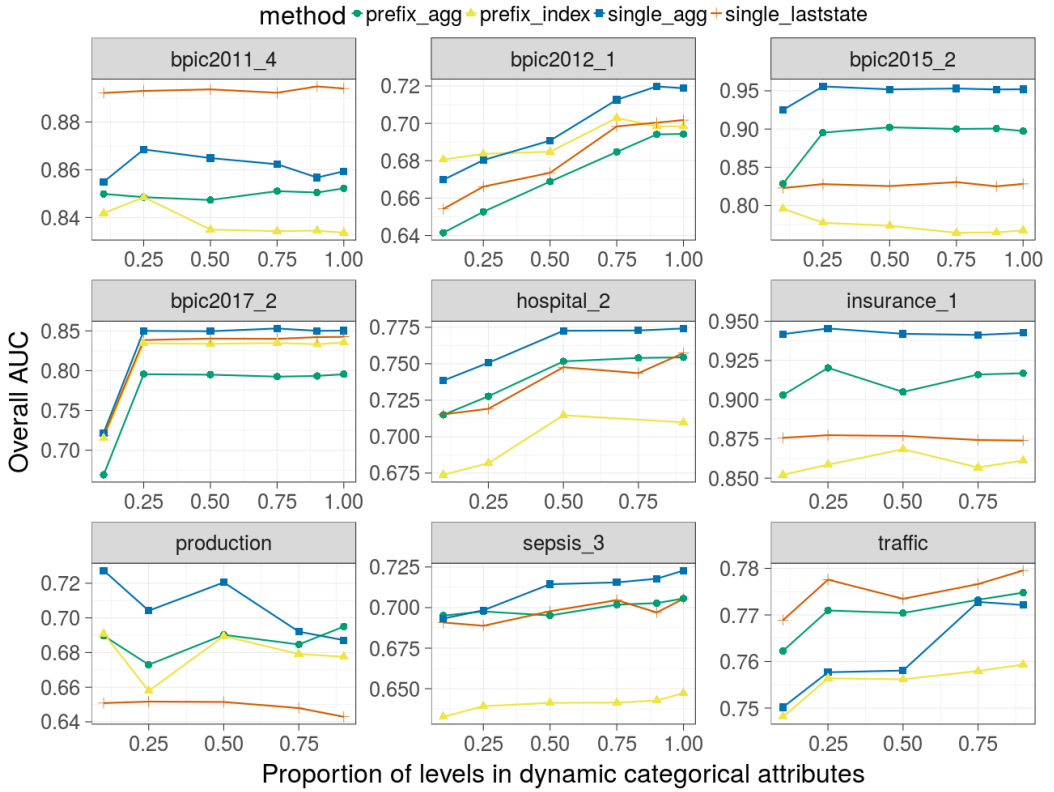
Fig. 13. AUC across different filtering proportions of dynamic categorical attribute levels (XGBoost)
