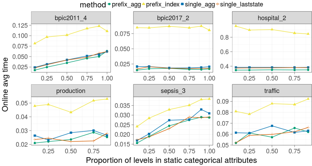
Fig. 25. Online times across different filtering proportions of static categorical attribute levels (XGBoost)
