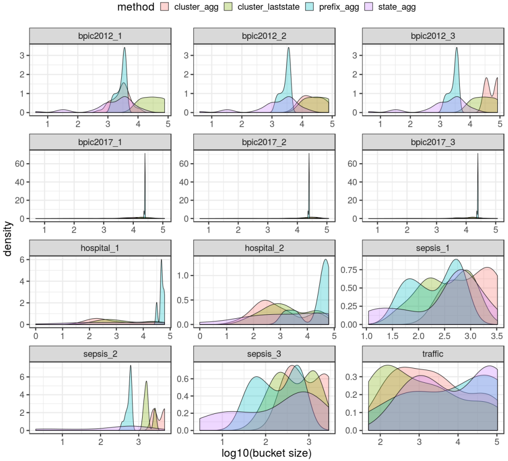
Fig. 18. Bucket size distributions (continued)
