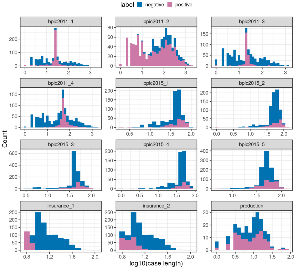
Fig. 15. Case length histograms for positive and negative classes
