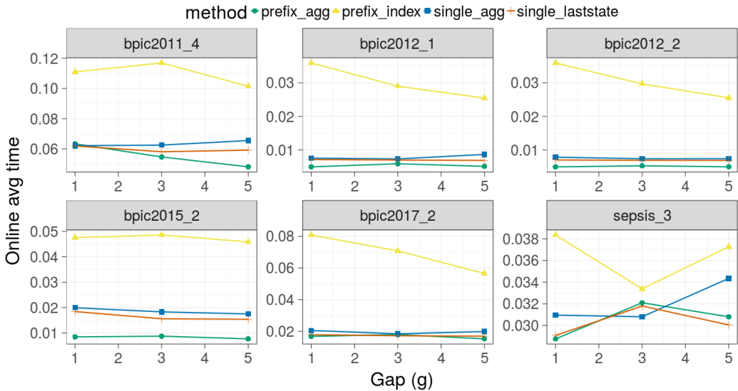
Fig. 11. Online times across different gaps (XGBoost)
