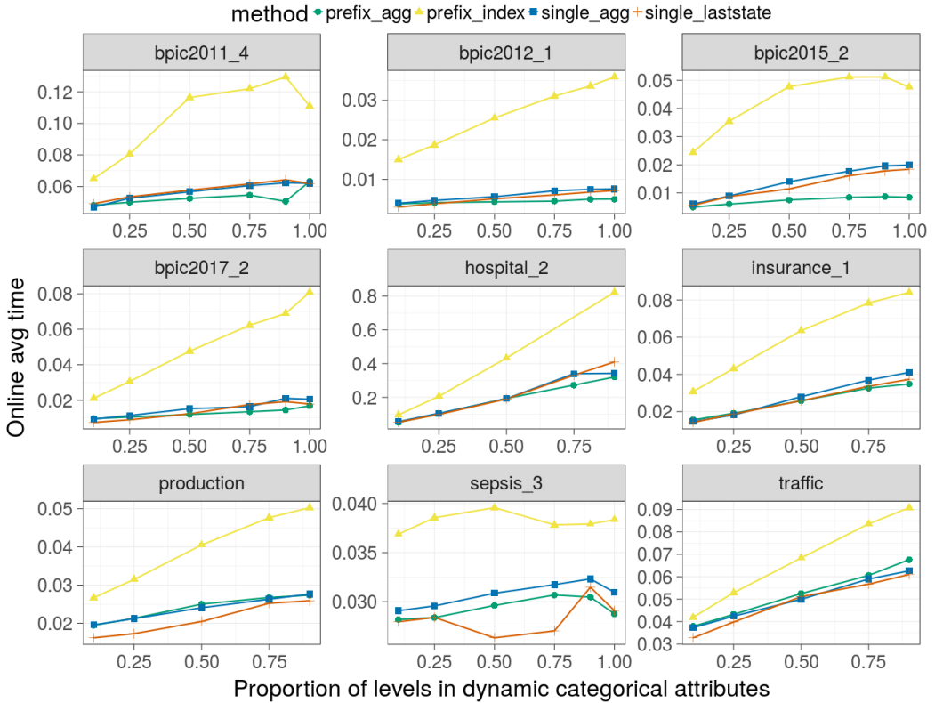
Fig. 14. Online times across different filtering proportions of dynamic categorical attribute levels (XGBoost)
