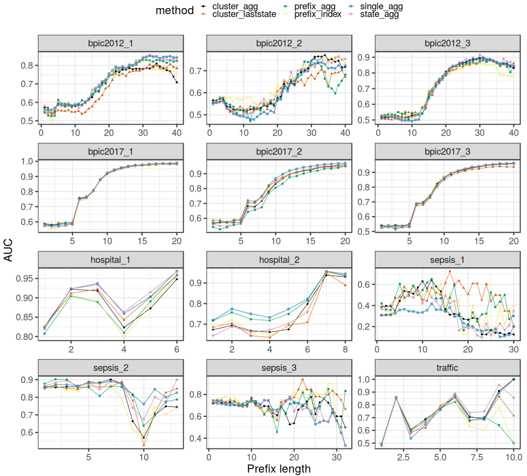
Fig. 8. AUC across different prefix lengths using XGBoost (continued)
