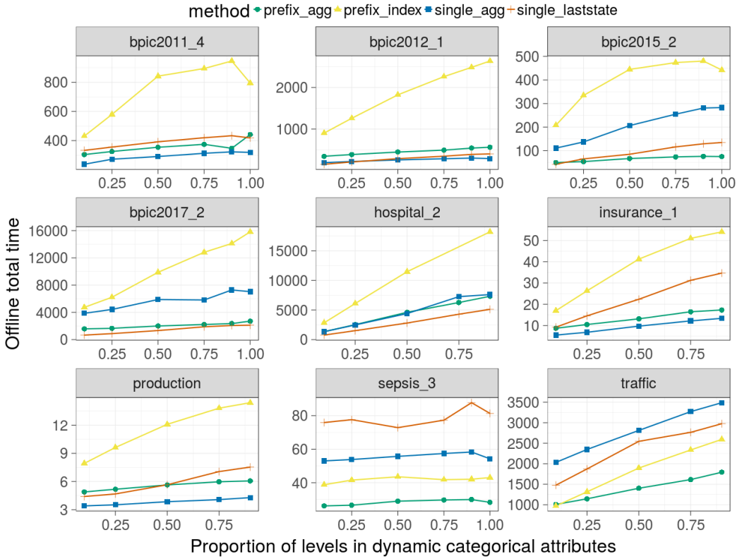
Fig. 12. Offline times across different filtering proportions of dynamic categorical attribute levels (XGBoost)
