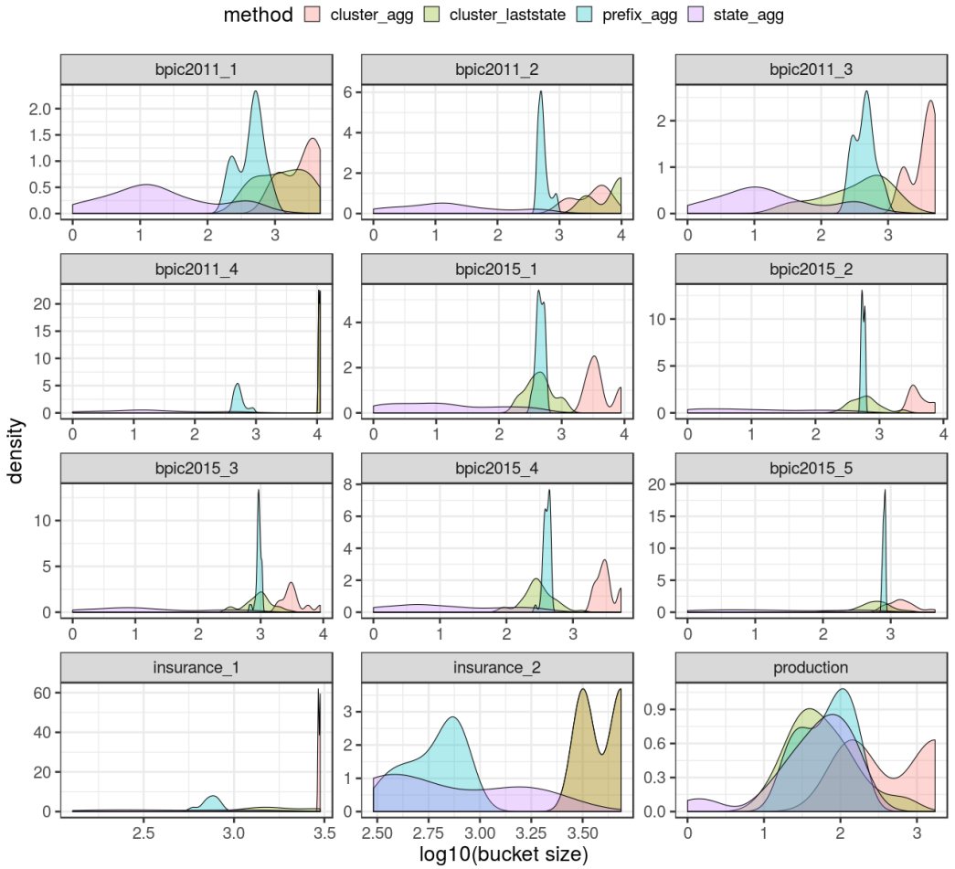
Fig. 17. Bucket size distributions
