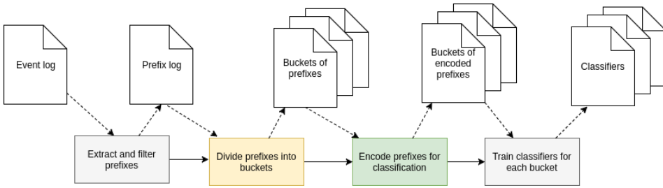
Fig. 2. predictive process monitoring workflow (offline phase)
