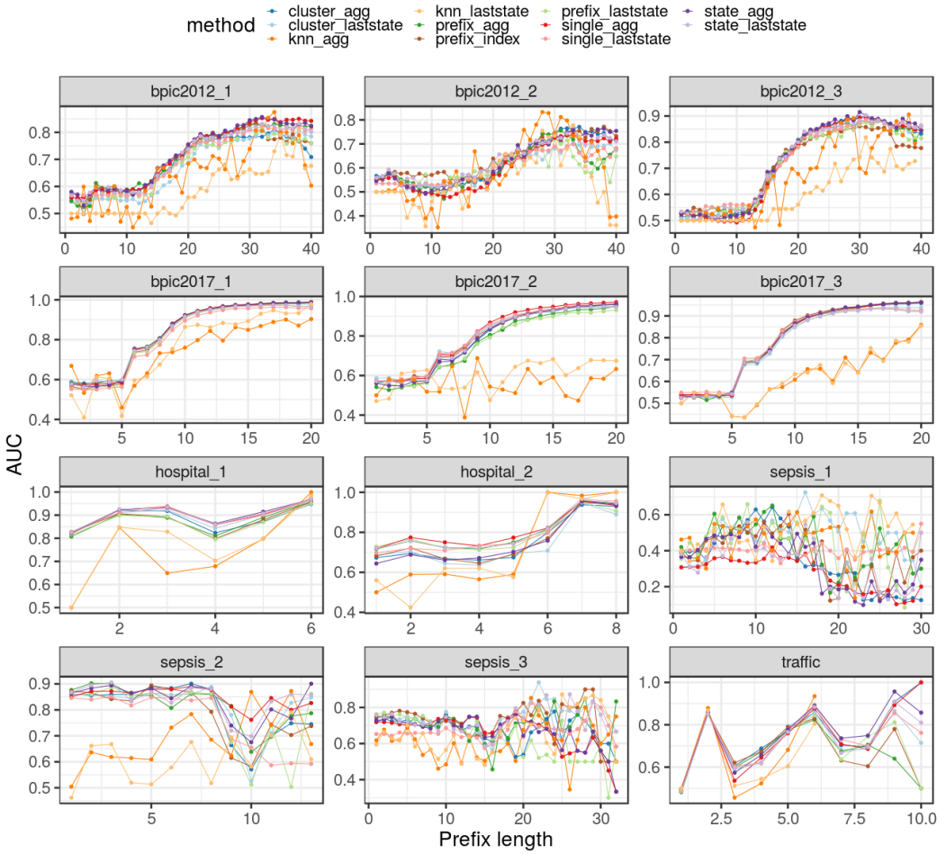
Fig. 20. AUC across prefix lengths using XGBoost, all methods (continued)
