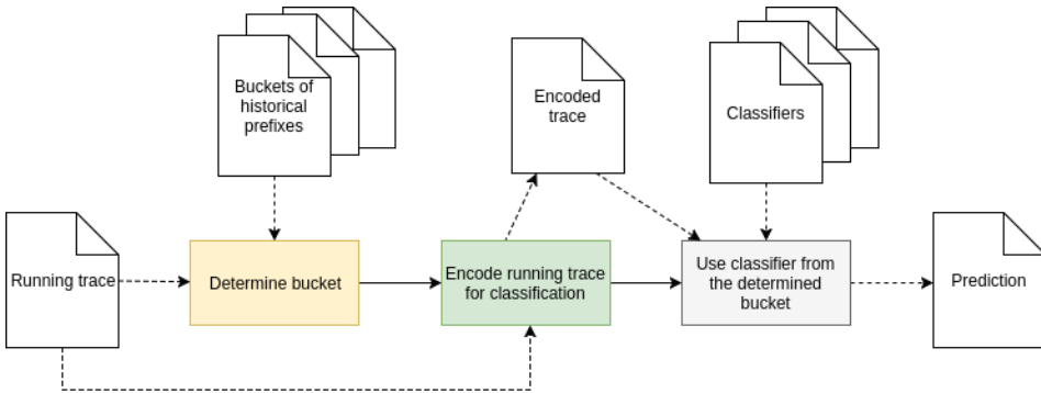
Fig. 3. predictive process monitoring workflow (online phase)
