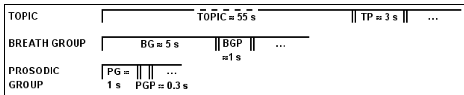
Fig. 6. A model of temporal structure of lecture speech
