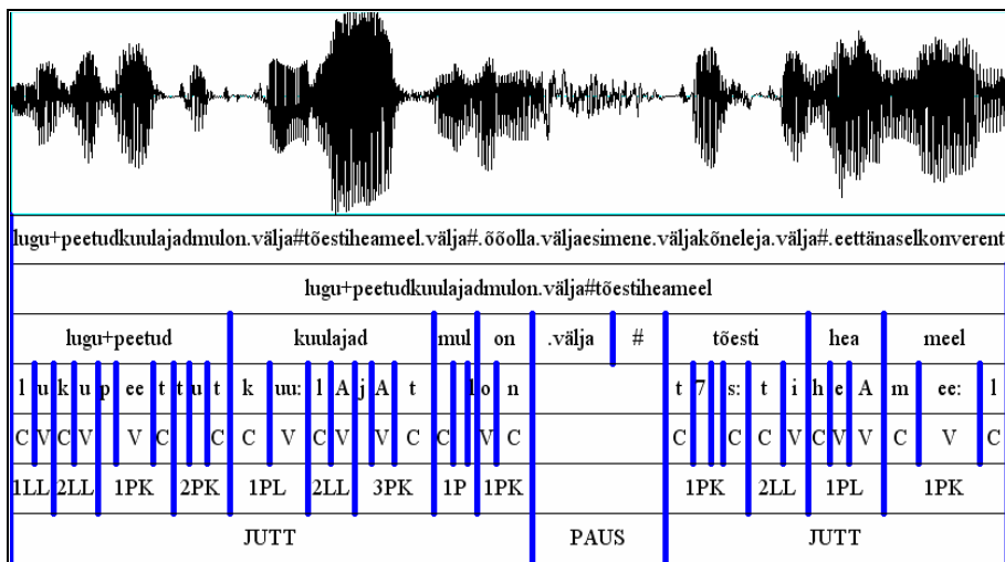
Fig. 1. An example of segmentation
